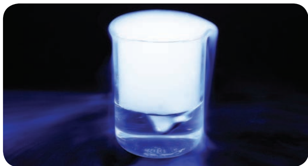
Figure 3.5 Solid carbon dioxide
