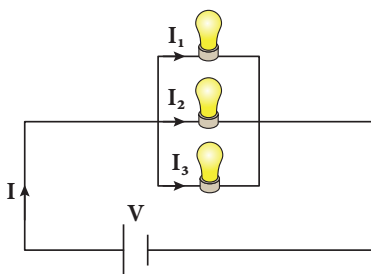
Figure 2.16 Current in parallel circuit
