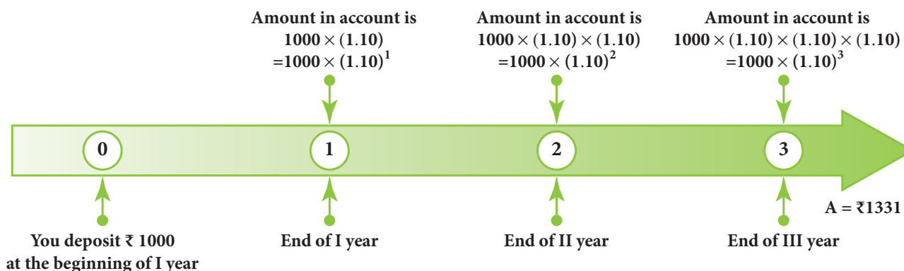
Flow chart showing 10% interest being compounded annually
