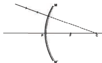
Figure 18 Rule 2
