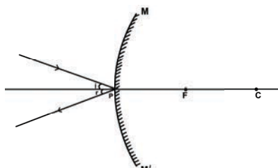
Figure 20 Rule 4
