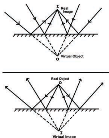
Figure 9 Real and virtual image
