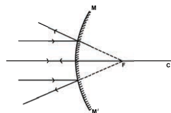
Figure 17 Rule 1
