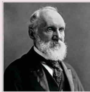
Lord kelvin
