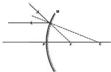
Figure 19 Rule 3
