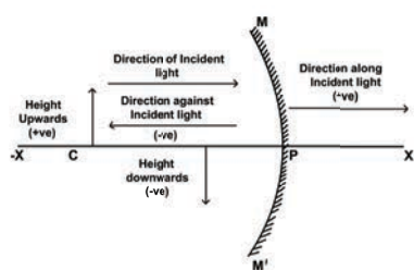
Figure 16 Sign convention for spherical mirrors
