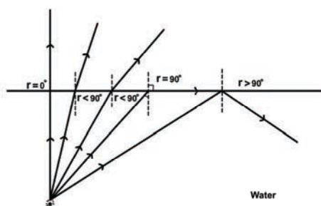
Figure 26 Critical angle
