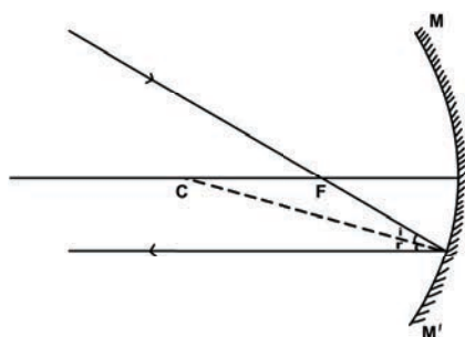
Figure 7 Ray travelling through the principal focus
