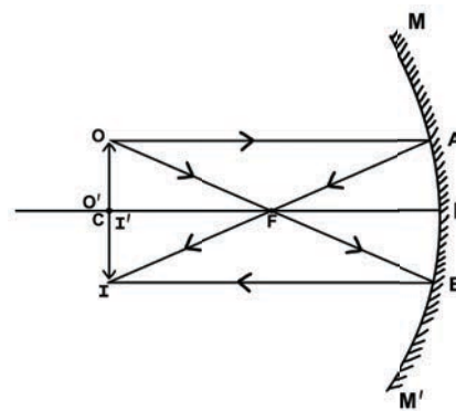
Figure 12 Object at the centre of curvature
