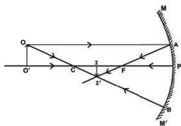
Figure 11 Object beyond the centre of curvature
