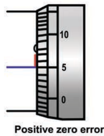
Figure 9 Positive Zero Error
