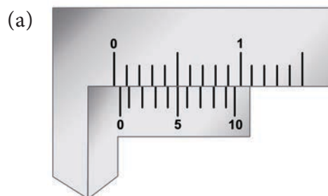
Positive zero error
