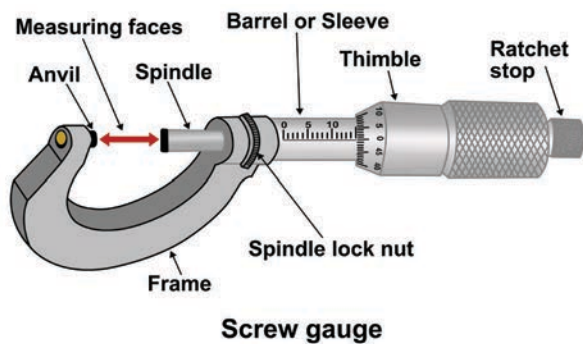
Figure 7 Screw gauge
