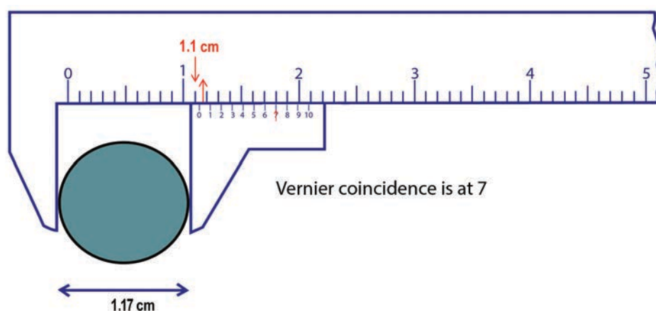
Figure 5 Measuring the diameter of a sphere
