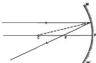
Figure 6 Ray parallel to principal axis
