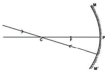
Figure 5 Ray passing centre of curvature
