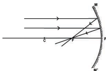
Figure 10 Object at infinity
