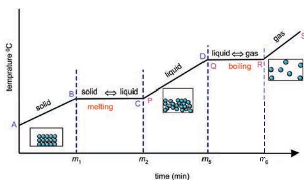
Changes of state — heating curve
