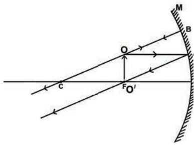
Figure 14 Object at principal focus
