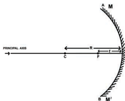
Figure 3 Concave mirror
