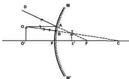
Figure 21 Image formation in a convex mirror
