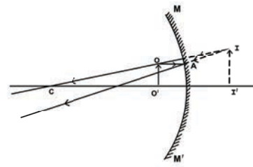
Figure 15 Object in between principal focus and pole
