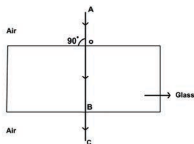
Figure 24 Incident of light ray in denser medium
