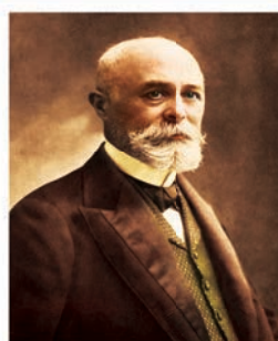
Henri Becquerel
