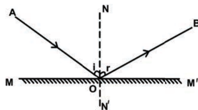
Figure 1 Plane mirror
