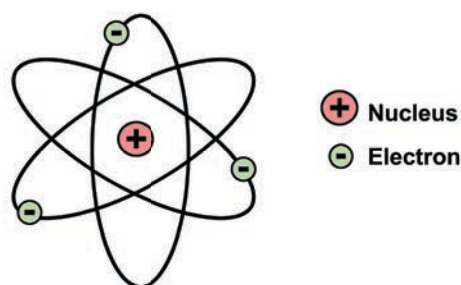
Rutherford Model of the Atom
