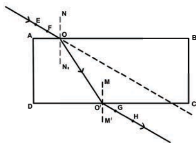
Figure 25 Verification of laws of refraction
