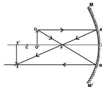
Figure 13 Object in between centre of curvature and principal focus
