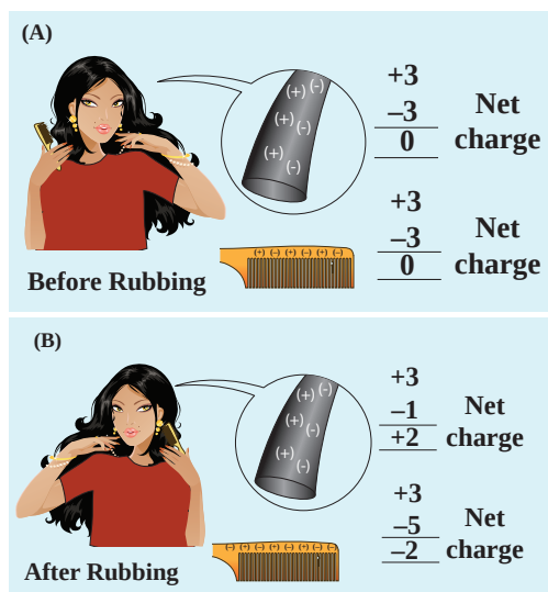
Figure 2.2 Frictional electricity
