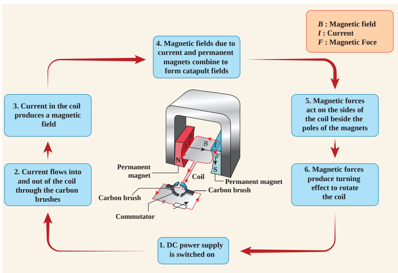
Figure 3.17 Principle of electric motor
