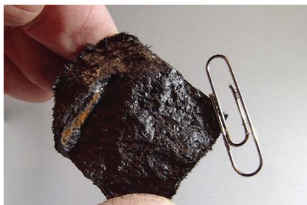
Figure 3.1 Natural magnets
