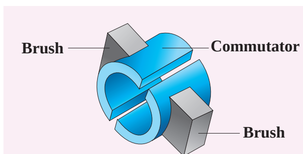
Figure 3.19 Close view of split ring and carbon brushes
